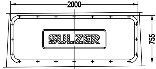
VIEW A 200 REMOVABLE ACCESS PANEL OPTIONAL
