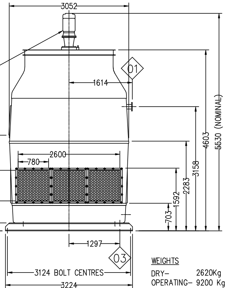
SIDE ELEVATION
